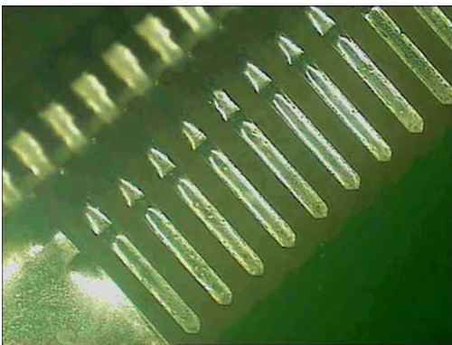
0.5mm pitch QFP(Profile view)
