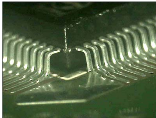
0.5mm pitch QFP
